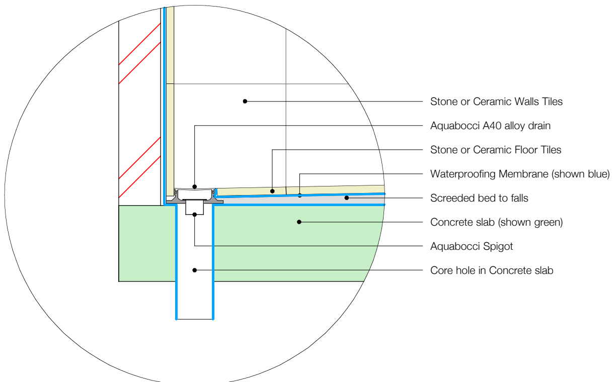
waterproofing detail scale 1:10
