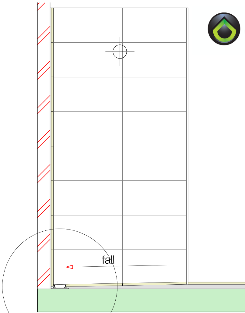
Shower wall section on concrete slab scale 1:20
